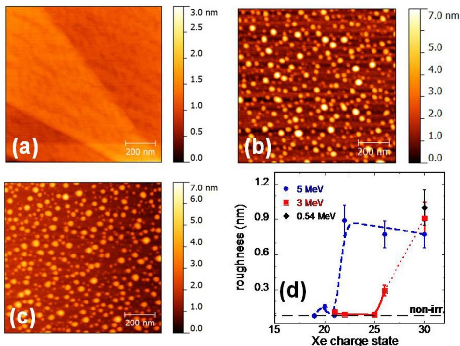
Figure 1 | \text{CaF}_2 surfaces irradiated by 5 MeV Xe ions with a fluence of 500 ions/ \mu\text{m}^2 . The AFM images show an area of 1 \times 1 \mu\text{m}^2 . A surface irradiated by (a) \text{Xe}^{21+} with no hillocks visible, (b) \text{Xe}^{22+} with \sim 520 hillocks, (c) \text{Xe}^{30+} with \sim 410 hillocks. (d) presents the evolution of the surface roughness versus charge state for samples before and after irradiation with 5, 3 and 0.54 MeV Xe ions. The lines are there to guide the eye.
