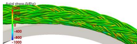
Figure 2: Detail of a braided rope bent over a sheave
