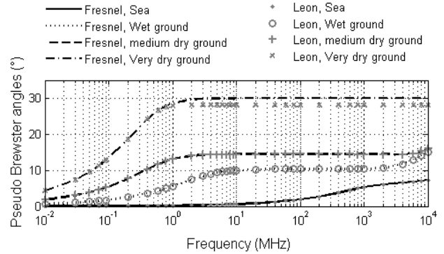
Fig. 5. For sea, wet ground, medium dry ground, very dry ground: variations of pseudo-Brewster angle with frequency modeled by Fresnel and Leontovitch reflection coefficient.
