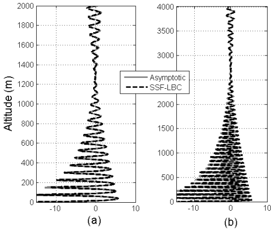
Fig. 3. Propagation factor (dB) vs altitude, at 1 GHz, V pol., distance 5 km, computed by asymptotic and SSF-LBC methods above (a) medium dry ground, (b) very dry ground.
