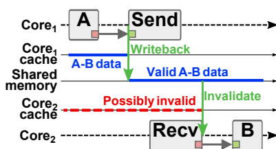
Fig. 4 Cache coherence solution without memory reuse
