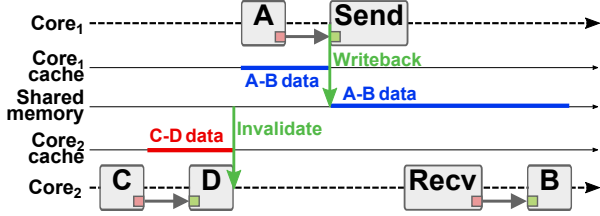
Fig. 16 Multicore cache coherence solution
