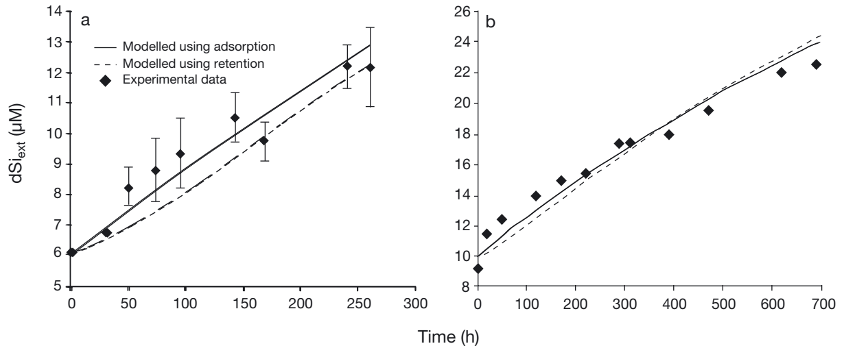
Fig. 1. Temporal evolution of the external silicic acid ( dSi_{ext} ) for (a) Skeletonema marinoi and (b) Chaetoceros decipiens from the adsorption (solid line) or the retention (dashed line) model version and experimental data (diamonds). Error bars in (a) are SE
