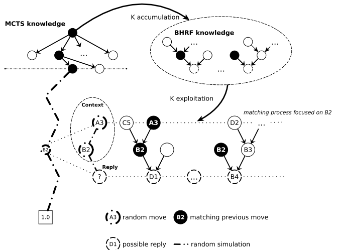
Figure 4: Background History Reply Forest process
