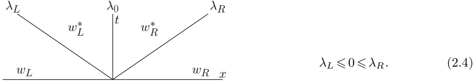
FIG. 2.1. Riemann solver.
