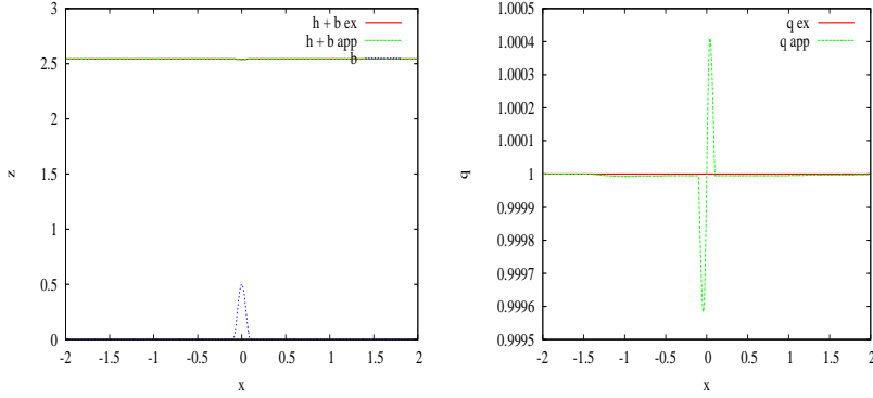
FIG. 3.4. Fluvial flow: Comparison of free surfaces h+b (left) and discharges q (right) resulting from the simple scheme (with suffix app) and the exact solution (with suffix ex) for a bottom topography b .
