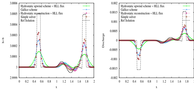
FIG. 3.1. Propagation of perturbations: Comparison of free surfaces h+b (left) and discharges q (right) for different schemes.
