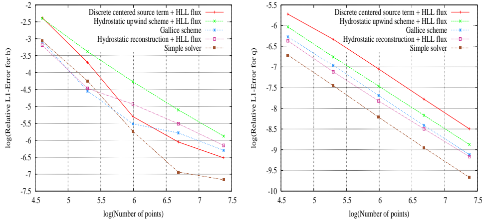
FIG. 3.7. Transcritical flow without shock: Comparison of orders of error for the water height h (left) and the discharge q (right) for different schemes.
