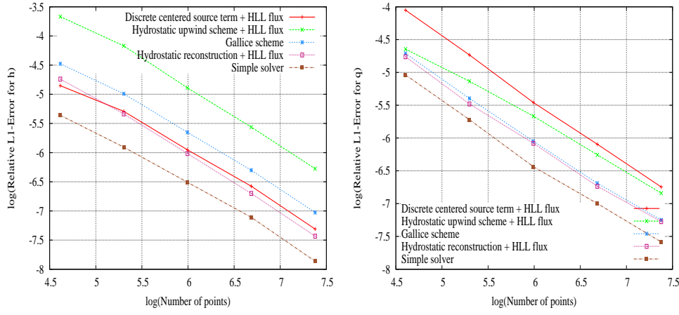
FIG. 3.9. Transcritical flow with shock: Comparison of orders of error for the water height h (left) and the discharge q (right) for different schemes.
