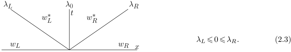
FIG. 2.1. Riemann solver.
