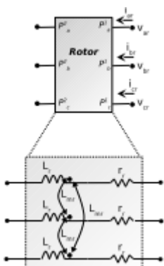
FIGURE 60 : ROTOR.
