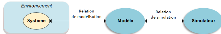
FIGURE 1 : FRAMEWORK M&S.
