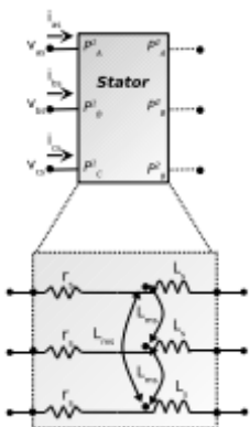
FIGURE 59 : STATOR.
