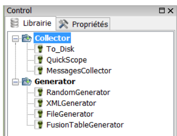
FIGURE 17 : LIBRAIRIES COLLECTOR ET GENERATOR.
