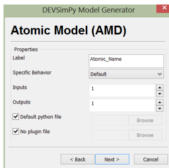
FIGURE 9 : INFORMATIONS.
