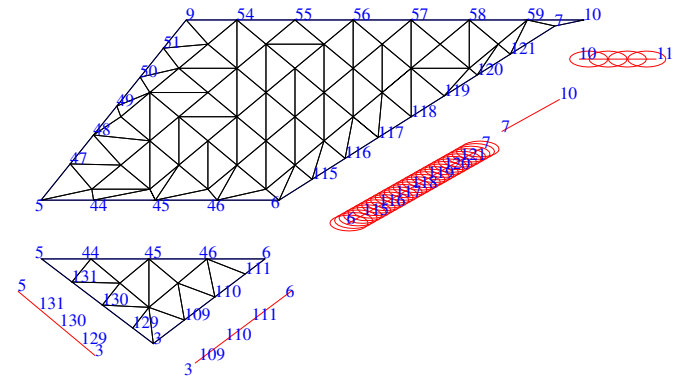
Fig. 5. Display of panels 1 and 3 showing finite element connectivity and assembly with surrounding cables.
