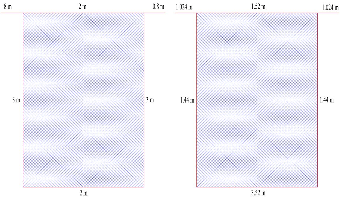
Fig. 14. Reference net (left) with dimensions 80 \times 120 in mesh units and optimized result (right). Cable lengths are indicated. One mesh out of two is displayed.
