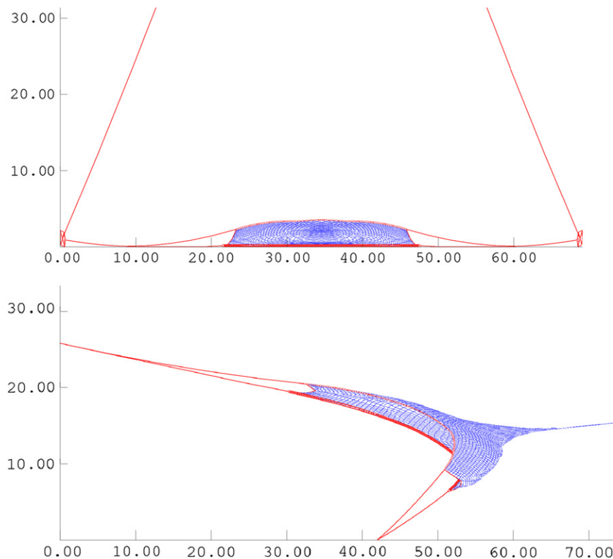
Fig. 8. Frontview (top) and 3D (bottom) aspects of the reference bottom trawl. We display a zoom on the netting and only one twine out of 10 are drawn. Since the top leg (cable #2 in Fig. 1) supports the entire fishing net, we expect its length to play a major role as discussed in the text.
