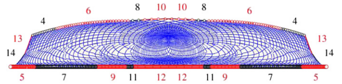
Fig. 7. Front view shape of reference trawl displaying cable number without ancillary rigging cables nor door structure (see Fig. 1). The numbering scheme is symmetric with respect to a vertical mirror plane situated at the center of the trawl. Only 1 twine out of 10 is drawn.
