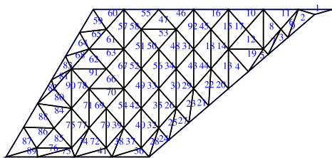
Fig. 4. Partitioning of panel number 3 into finite elements with numbering scheme. The mesh discretization size is 2 m on the left and 0.5 m on the right where nodes are displayed.
