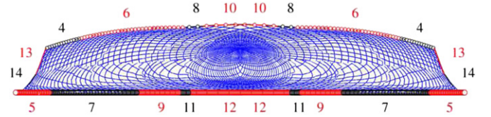
Fig. 7. Front view shape of reference trawl displaying cable number without ancillary rigging cables nor door structure (see Fig. 1). The numbering scheme is symmetric with respect to a vertical mirror plane situated at the center of the trawl. Only 1 twine out of 10 is drawn.
