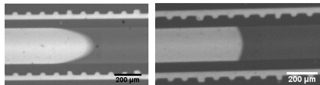
Figure 4: Optical images of ethanol contact angle before (left) and after (right) FDTS deposition (microchannel of 20µm depth). The liquids appears in dark.
