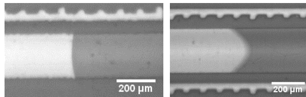
Figure 2: Optical images of water contact angle before (left) and after (right) SiO 2 deposition (microchannel of 20µm depth). The liquids appears in dark.
