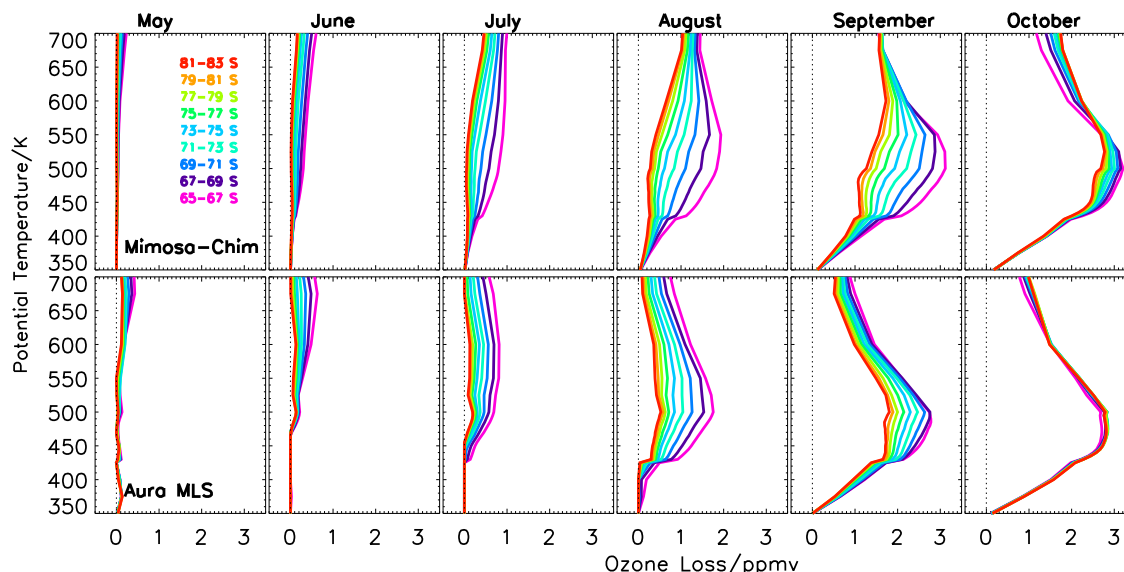
Figure 1. The 10-year (2004–2013) average monthly mean ozone loss estimated at different equivalent latitude (EqL) bins (of 2^\circ ) from 65 to 83^\circ S EqL from the MIMOSA–CHIM simulations and MLS measurements. The model results are interpolated with respect to the time and location of the MLS measurements inside the vortex and then averaged for the corresponding day. The y axis represents potential temperature in K. The black dotted lines represent 0 ppmv.
