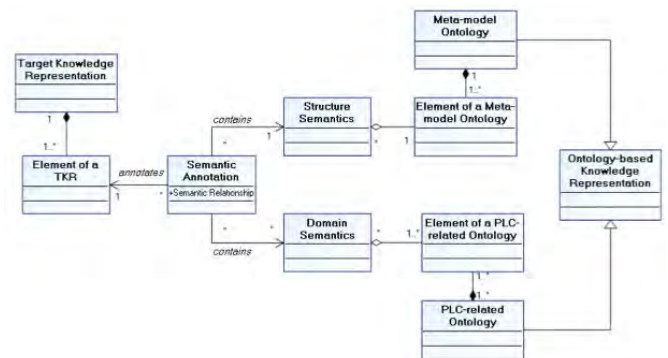
Figure 1. The Meta-model of the Semantic Annotation
