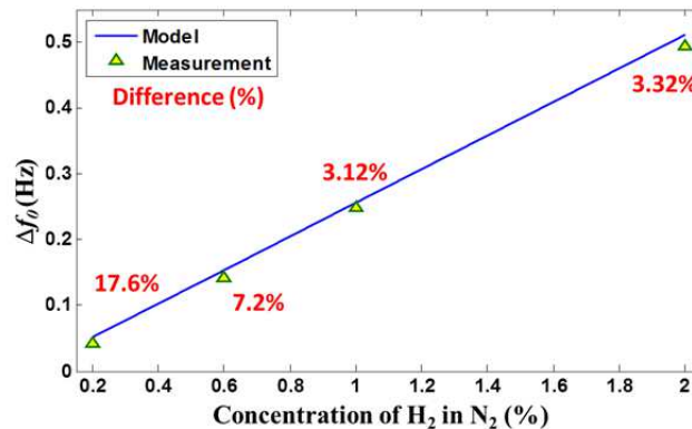
Fig. 7 : Measurement of concentration of H 2 in N 2 (0.2-2%) with gas flow of 100 ml/min using rectangular-shaped microcantilever ( L \times b \times h = 2000 \times 400 \times 5 \mu\text{m}^3 ). The triangle markers present experimental measurements, the blue line presents the theoretical modeling [Eq. (3)] and the red numerical values present the relative deviation between model and measurements.
