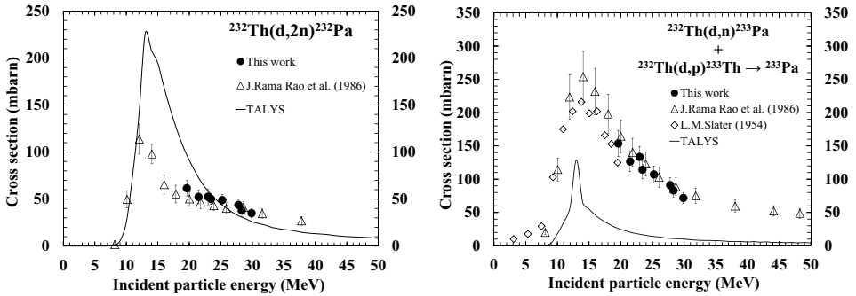
Fig. 2. Production cross section of ^{232}\text{Th}(d,n)^{232}\text{Pa} (on the left) and cumulative production cross section of ^{233}\text{Pa} (on the right).
