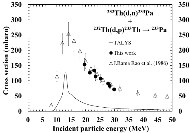
FIG. 3. Cumulative production cross section of ^{233}\text{Pa} .
