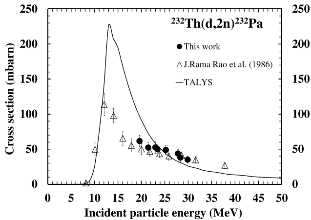
FIG. 2. Experimental cross section of ^{232}\text{Th}(d,2n)^{232}\text{Pa} .
