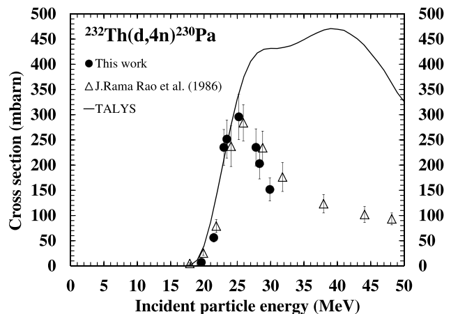
FIG. 1. Experimental cross section of ^{232}\text{Th}(d,4n)^{230}\text{Pa} .
