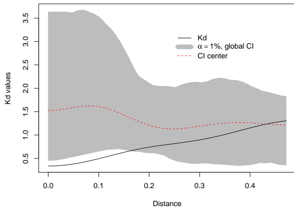
(a) K_d function results
