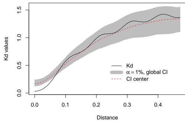
(c) K_d results for regular distribution of cases (map on figure 3a) with the original Duranton and Overman's smoothing
