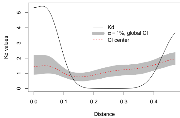
(b) K_d results for aggregate distribution of cases (map on figure 2a)
