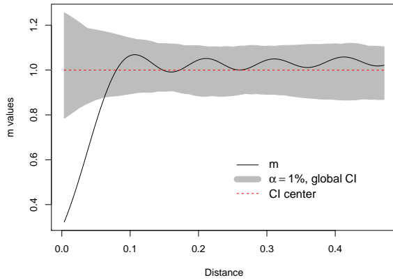
(b) m function results, original bandwidth of Silverman (1986)
