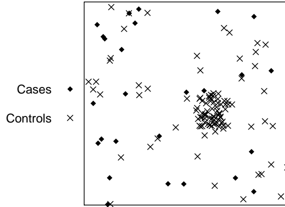
Figure 5. A more complex theoretical case
