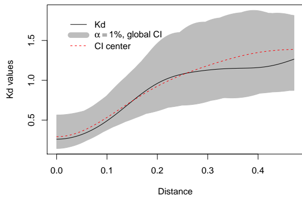
(a) K_d results for completely random distributions of cases and controls (map on figure 1a)
