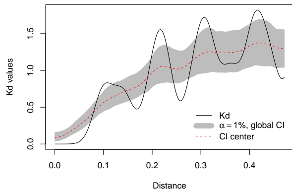
(d) K_d results for regular distribution of cases (map on figure 3a) with a more detailed smoothing
