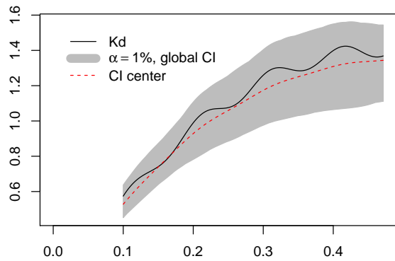
(c) K_d results for regular distribution of cases (map on figure 3a) with the original Duranton and Overman's smoothing
