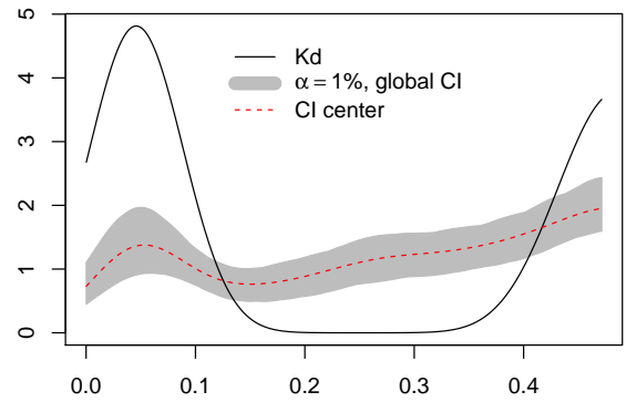
(b) K_d results for aggregate distribution of cases (map on figure 2a)
