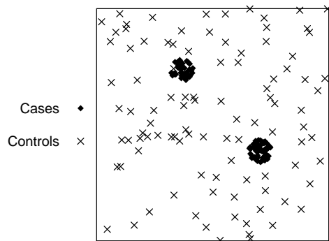
(a) Aggregate distribution of cases, complete spatial randomness for controls
