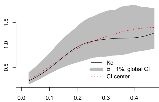
(a) K_d results for completely random distributions of cases and controls (map on figure 1a)
