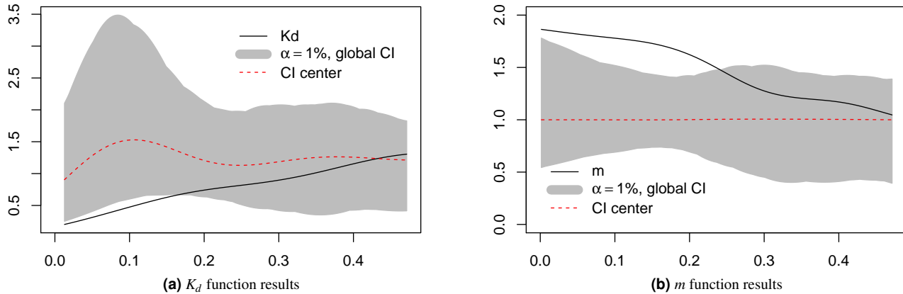
Figure 6. K_d and m results for a more complex theoretical case
