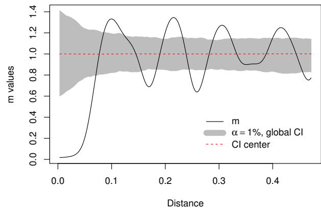
(c) m function results, half of the original bandwidth of Silverman (1986)
