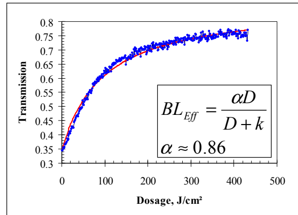
Fig. 5. Evolution of the Nd:YAG laser power transmitted through the PTR glass being bleached as a function of the dosage of exposure for an energy per pulse of 1.05 J/cm 2 and its fit using an hyperbolic function.
