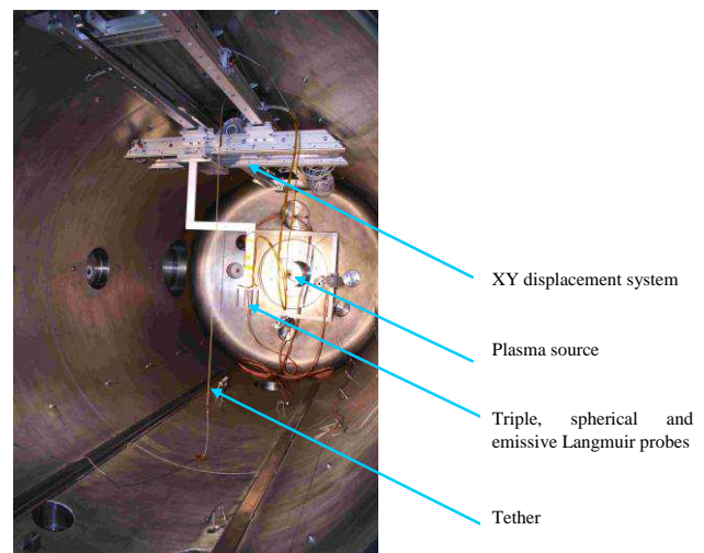
Fig. 1. Experimental setup for current collection measurement
