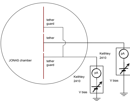
Fig. 3. Electrical circuit for current collection measurement
