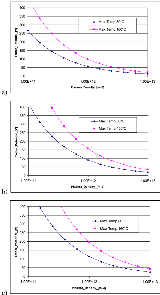
Fig. 6. Maximum operational tether potential as a function of the plasma density for a) \epsilon_s = 0.03 , b) \epsilon_s = 0.06 and c) \epsilon_s = 0.085
