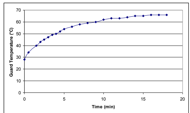
Fig. 4. Guard sample temperature after 20 min of current collection at +200V for a plasma source at 20V – 1mA.
