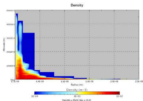
Figure 8 : Density of dust above the simulation domain, as a function of altitude and dust radius.
