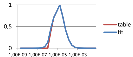
Figure 3 : Distribution of the dust radii (m) from the table given in [4] and the fit in used in SPIS.
