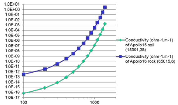
Figure 2: Bulk conductivities ( \text{ohm}^{-1} \cdot \text{m}^{-1} ) of two lunar samples as a function of the temperature (K), from [4].
