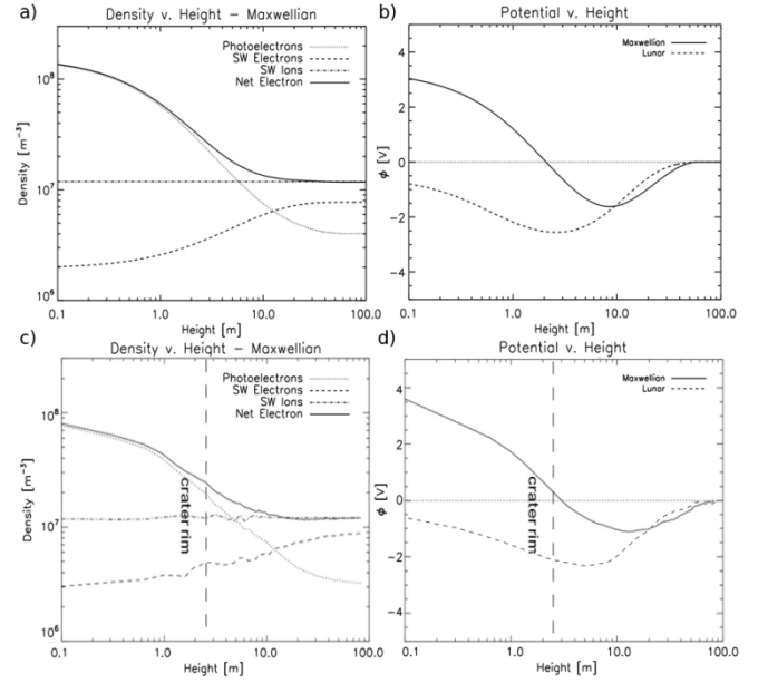
Figure 4: Density (a,c) and potential (b,d) profiles for the simulation of [7] and the test case, respectively.
