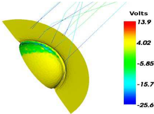
Figure 5: Surface potential and test-particle dust trajectories
