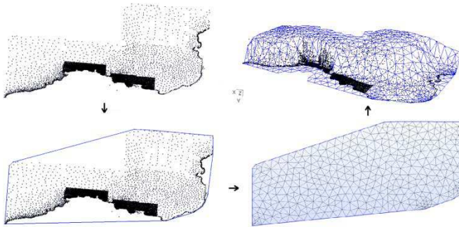
Figure 1: Definition of the lunar surface mesh from a list of ground coordinates.
