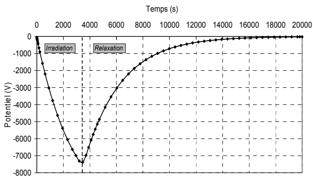
Fig. 12. Evolution of surface potential on a 127 \mu\text{m} thick Kapton® piece in 1 hour worst case irradiation conditions, preceded by the IGE spectrum for 1 day (radiation history)
