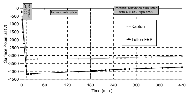
Fig. 10. Evolution of surface potential measured on Kapton® and Teflon® at -150^{\circ}\text{C} during three different phases : 1. under mono-energetic 20 keV electron irradiation, 2. during intrinsic relaxation, 3. during relaxation stimulated with 400 keV electron beam (flux : 1\text{ pA}\cdot\text{cm}^{-2} )
