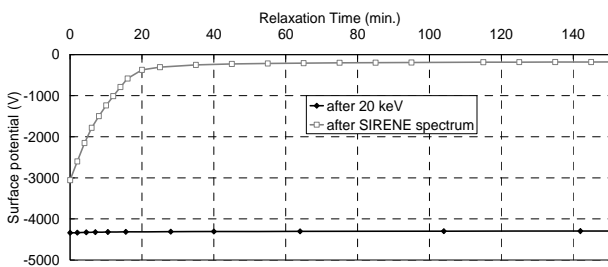
Fig. 8. Evolution of surface potential on 127 \mu\text{m} thick Teflon FEP sample after 20 keV electron irradiation or GEO like SIRENE spectrum
