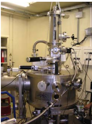
Fig. 2. View of the SPIDER facility
