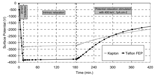
Fig. 9. Evolution of surface potential measured on Kapton® and Teflon® at -30^{\circ}\text{C} during three different phases : 1. under mono-energetic 20 keV electron irradiation, 2. during intrinsic relaxation, 3. during relaxation stimulated with 400 keV electron beam (flux : 1\text{ pA}\cdot\text{cm}^{-2} )
