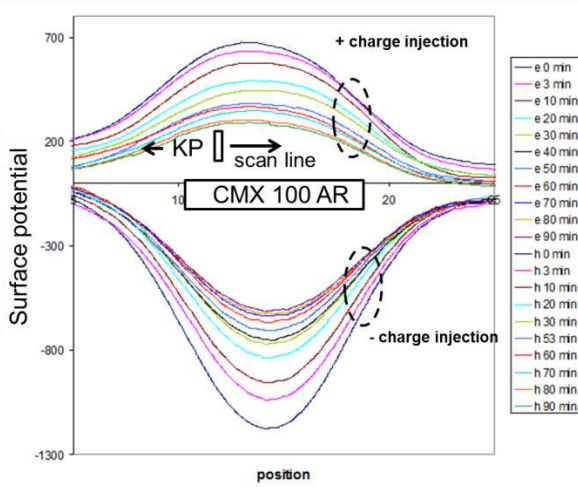
Fig. 4. Surface potential profiles measured on CMX 100 AR during the charge relaxation and after positive and negative charge injection (h= holes injection and e=electrons injection).
