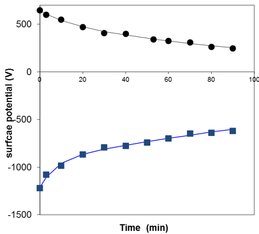
Fig. 5. Surface potential versus time on CMX 100 Ar during the charge relaxation after negative (bleu) and positive (black) charge injection
