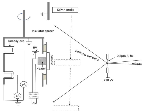
Fig. 1. CEDRE Facility
