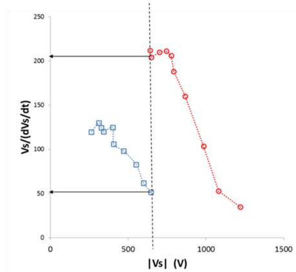
Fig. 6. V_s/(dV_s/dt) curves as function of the magnitude of the surface potential after negative (red) and positive (bleu) charging.
