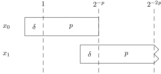
Figure 1. Schematic representation of the decomposition x = [x_0, x_1] = x_0 + x_1 .
