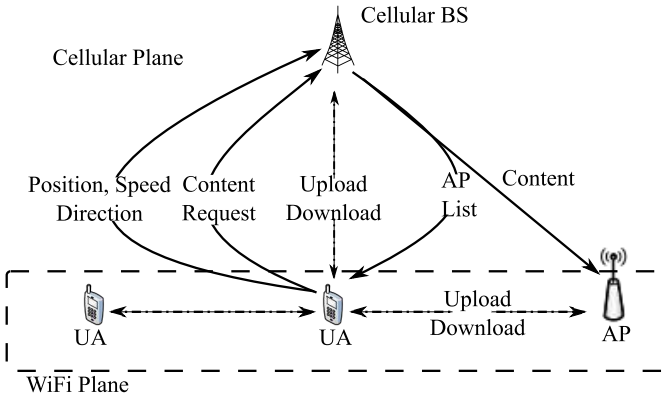
Fig. 8. MADNet system architecture [5]: when a mobile node wants to communicate, it makes a request to the cellular BS, which may reply directly forwarding the content through the cellular network or sending the content to a neighboring AP. The BS predicts the route of the nodes using the status information sent by the mobile node.
