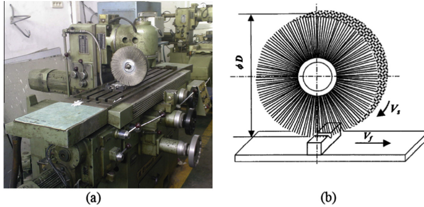
Fig. 3. Wire brush hammering apparatus, (a) experimental setup, and (b) schematic form of wire brush hammering.
