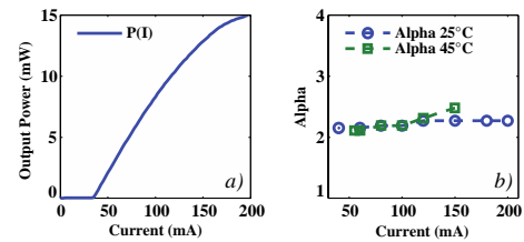
Fig.1: Static characteristics of p-doped QDash laser a L(I) characteristics of the DFB laser under evaluation at room temperature b Measured \alpha -parameter constant over large range of current both at room temperature and in semicooled operation
