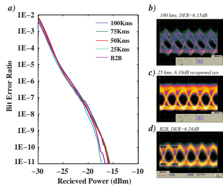
Fig4: Optical transmission using on Etalon filter
