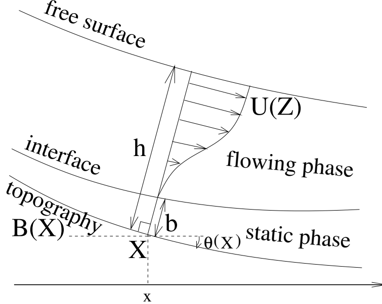
Figure 2: Generic velocity profile for viscoplastic flows with static/flowing interface. The tangential velocity U has a static part 0 < Z < b and a flowing part b < Z < h , separated by an interface b , where h is the thickness of the granular layer. The case \theta < 0 and \partial_Z U > 0 is represented.
