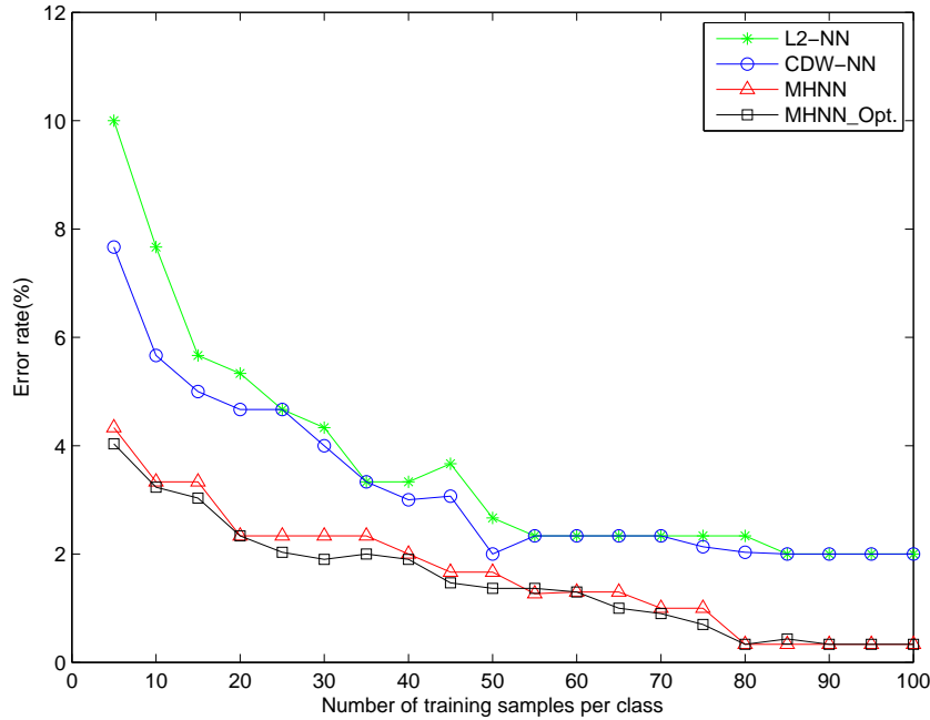
Figure 3: Classification error rates of our proposed method in comparison with other methods with different training set sizes.
