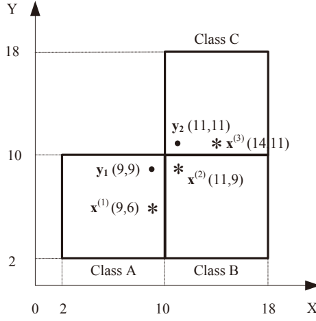
Figure 1: A three-class classification example.
