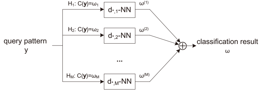
Figure 2: General scheme of the MHNN classifier
