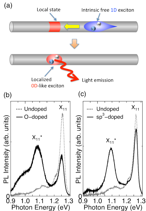
Figure 1. (a) Schematic of exciton dynamics in a SWNT with a 0D-like local luminescent state. Intrinsic free 1D exciton diffusively moves along the nanotube axis, converted to a 0D-like exciton at the local state, and emit brighter PL than 1D excitons. (b, c) PL spectra of SWNTs measured with an excitation photon energy of 2.18 eV before (dotted curve) and after (solid curve) the doping of (b) oxygen and (c) sp 3 -defect, respectively. The dominant peak at ~1.25 eV ( E_{11} ) corresponds to PL from the intrinsic first subband excitons ( X_{11} ) in (6,5) SWNTs. The new peaks at ~1.05-1.10 eV ( E_{11}^* ) in (b) and (c) are attributed to PL from the 0D-like excitons ( X_{11}^* ) trapped at local quantum states embedded in SWNTs.
