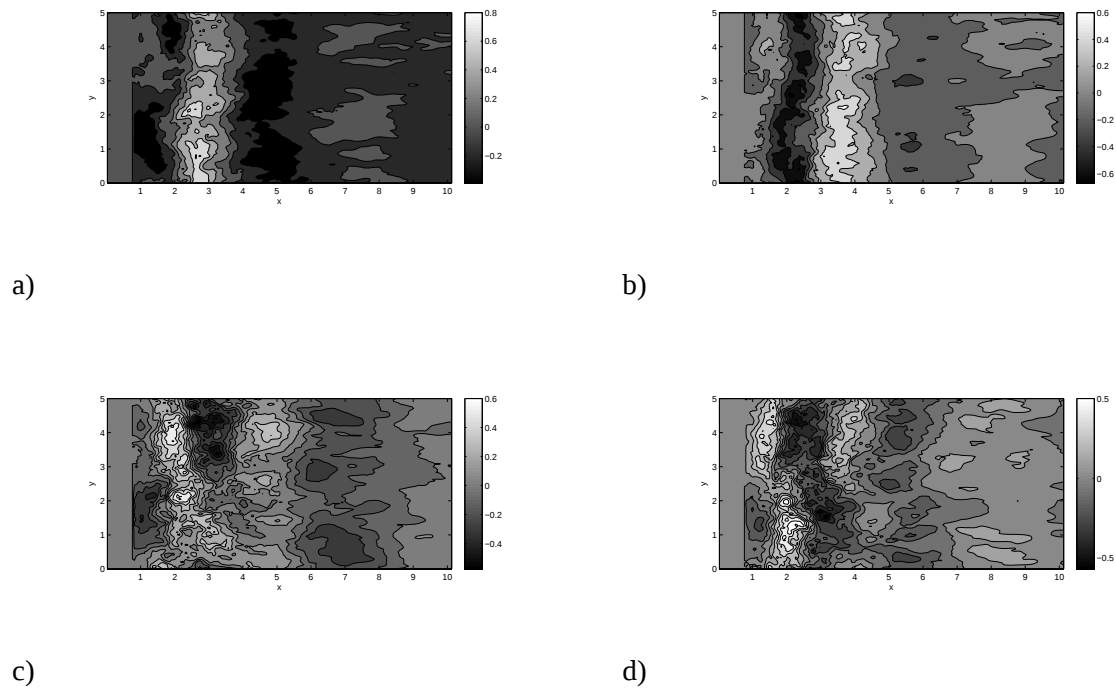
Figure 7: Pressure POD mode a) n = 2 b) n = 3 c) n = 4 d) n = 5 .
