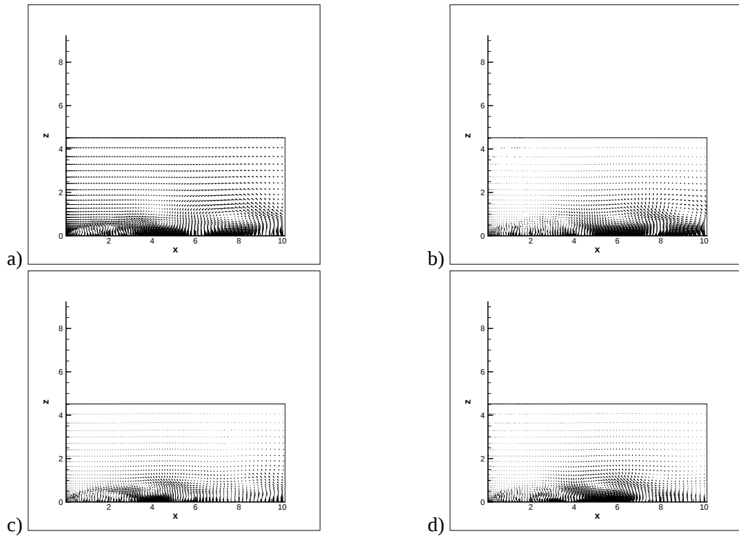
Figure 9: Spanwise-averaged full POD velocity mode a) n = 2 b) n = 3 c) n = 4 d) n = 5
