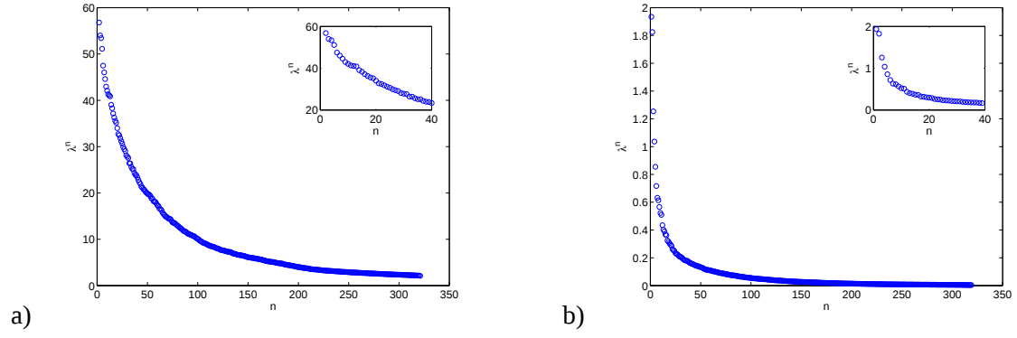
Figure 2: a) POD spectrum of the full field b) POD spectrum of the wall pressure.
