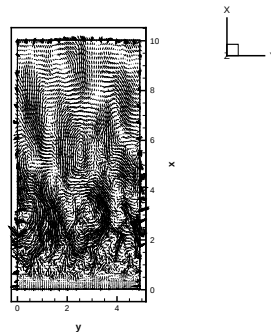
Figure 5: Horizontal view of the second velocity POD mode at z = 0.4H .
