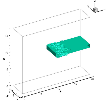
Figure 1: Isosurface of zero streamwise velocity- the arrow indicates the flow direction.
