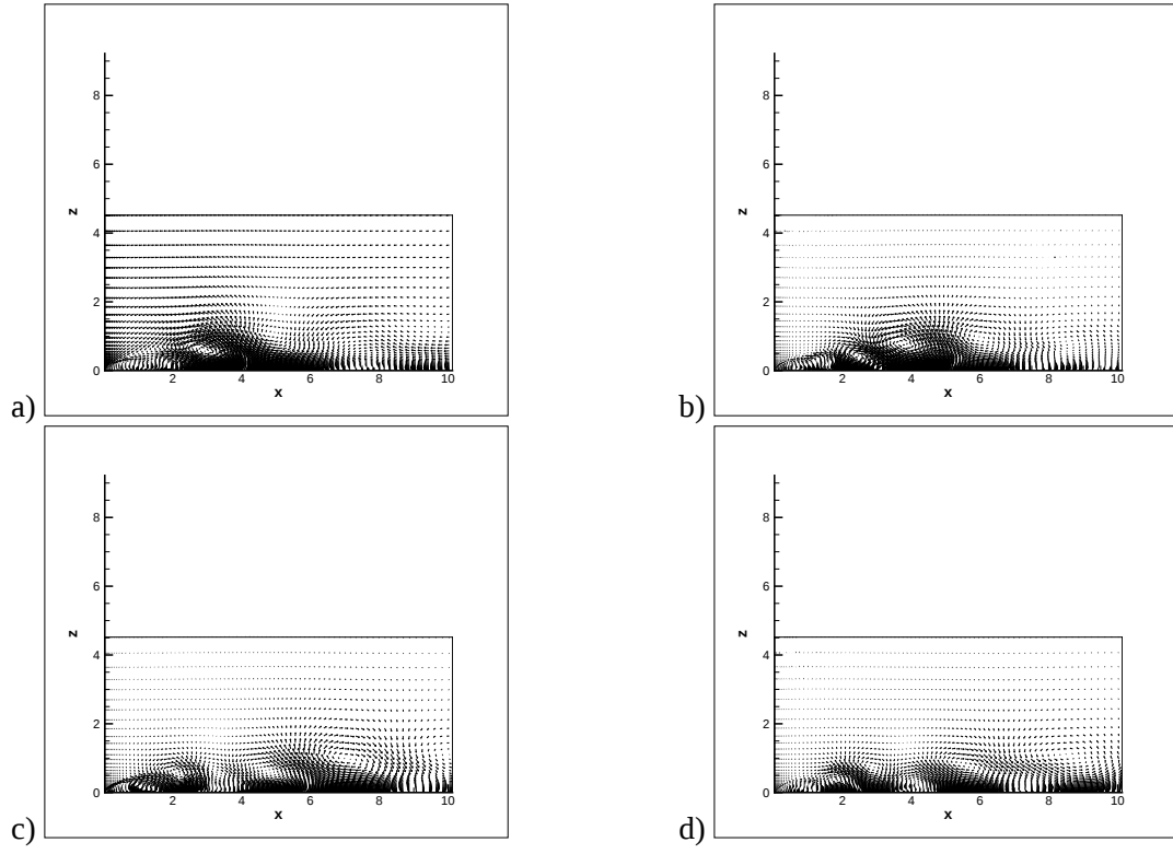
Figure 8: Pressure-educed spanwise-averaged velocity mode a) n = 2 b) n = 3 c) n = 4 d) n = 5 .
