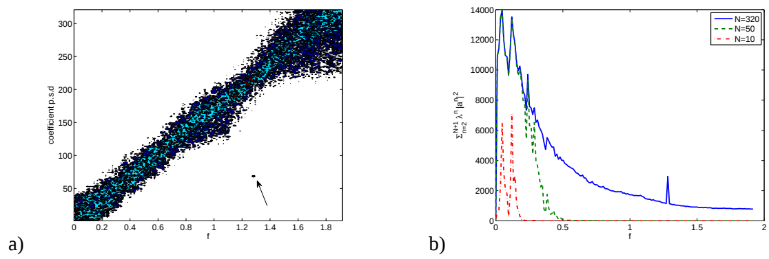
Figure 3: The frequency is adimensionalized with the plate thickness a) Spectral density of the pressure POD coefficients a_p^n . The arrow indicates the location of the Kelvin-Helmholtz frequency b) Spectral density of the POD energy \sum_{n=2}^{N+1} \lambda^n |\hat{a}^n(f)|^2 .
