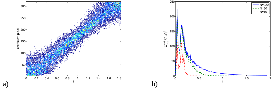
Figure 6: The frequency is adimensionalized with the plate thickness a) Spectral density of the pressure POD coefficients a_p^n b) Spectral density of the POD energy \sum_{n=2}^{N+1} \lambda^n |\hat{a}_p^n(f)|^2 .
