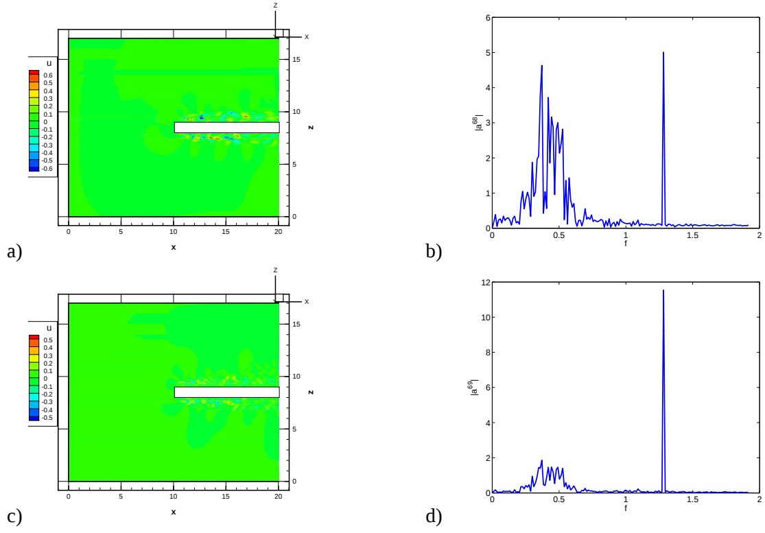
Figure 4: Modes associated with the frequency fH/U_0 = 1.2 a) cross-section y = 0 of streamwise velocity \phi_u^n for n=68 b) spectral density of a^{68} c) cross-section y = 0 of streamwise velocity \phi_u^n for n=69 d) spectral density of a^{69} .
