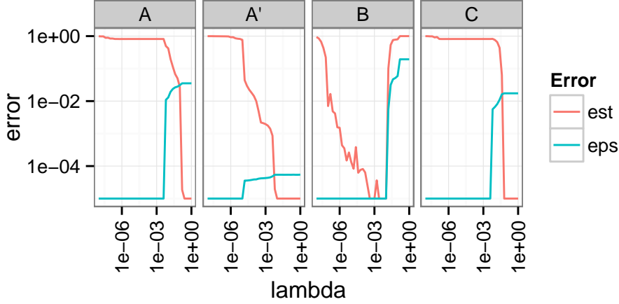
FIGURE 5.2. Error versus regularization parameter \lambda . Problems details are given in the main text. Estimation error ( est ) is given in (5.1). Epsilon error ( eps ) is the value of \epsilon in program (iocp). Trajectory sample size: 20 for A, A' and B, 50 for C. Degrees of l and v are 4 and 10 respectively.
