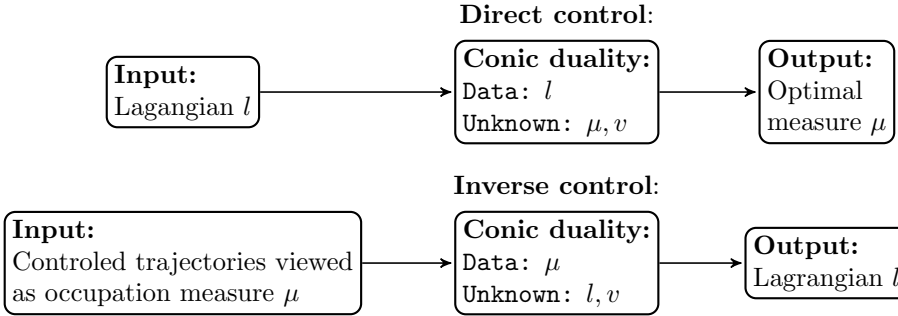
FIGURE 1.1. Direct optimal and inverse optimal control flow chart. System description is given by the dynamics f , the state constraint set X and control constraint set U which are all assumed to be fixed. We emphasize that the Lagrangian and the occupation measure have symmetric roles for the direct and inverse problems. We also note that the output of the inverse problem is a Lagrangian. Solving the direct optimal control problem for new initial conditions is an important question but remains secondary regarding inverse optimality which is the focus of this work.
