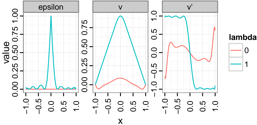
FIGURE 5.1. Solution for the one dimensional minimum exit time problem, effect of the regularization parameter \lambda . See Section 5.2 for problem details and comments. The first column is the distribution of the error \epsilon . It represents the value of l(x, u) + \text{grad } v \cdot f(x, u) as a function of x where u = \text{sign } x is the optimal control. The second column is a representation of the value function v and the third column is a representation of its derivative for solutions of problem (iocp) with and without regularization. We take 100 points on the segment. Lagrangian l and value function v are both polynomials of degree 16.
