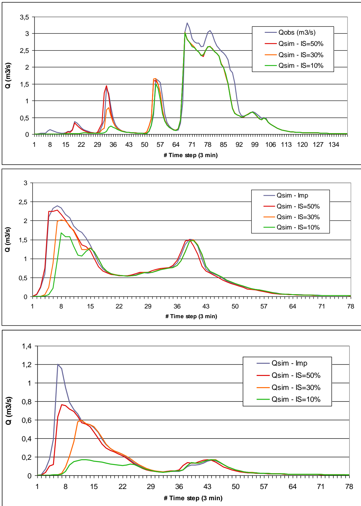
Figure 2. Simulation results obtained for 14/07/2010 (top), 12/06/2010 (middle) and 22/07/2011 (bottom) events: Qsim-Imp corresponds to the current situation (without any green roof) and Qsim-IS=50%, Qsim-IS=30% and Qsim-IS=10% to green roof situations characterized by an initial saturation of the substrate of about 10, 30 and 50%.
