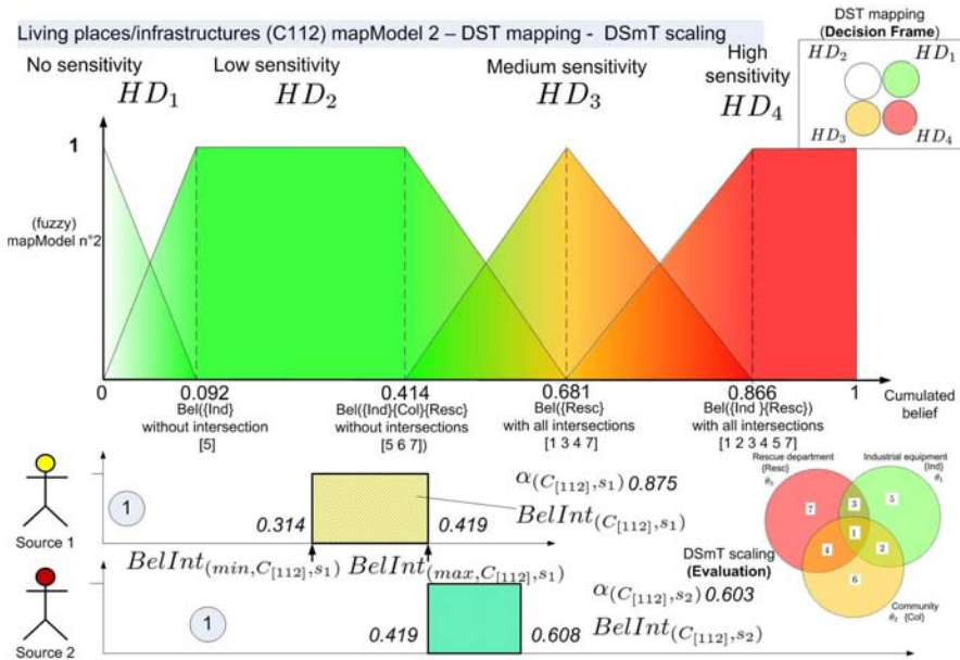
Figure 23.50: Qualitative criterion C_{[112]} - DST mapping - DS m T scaling - Evaluation intervals for sources 1 and 2.
