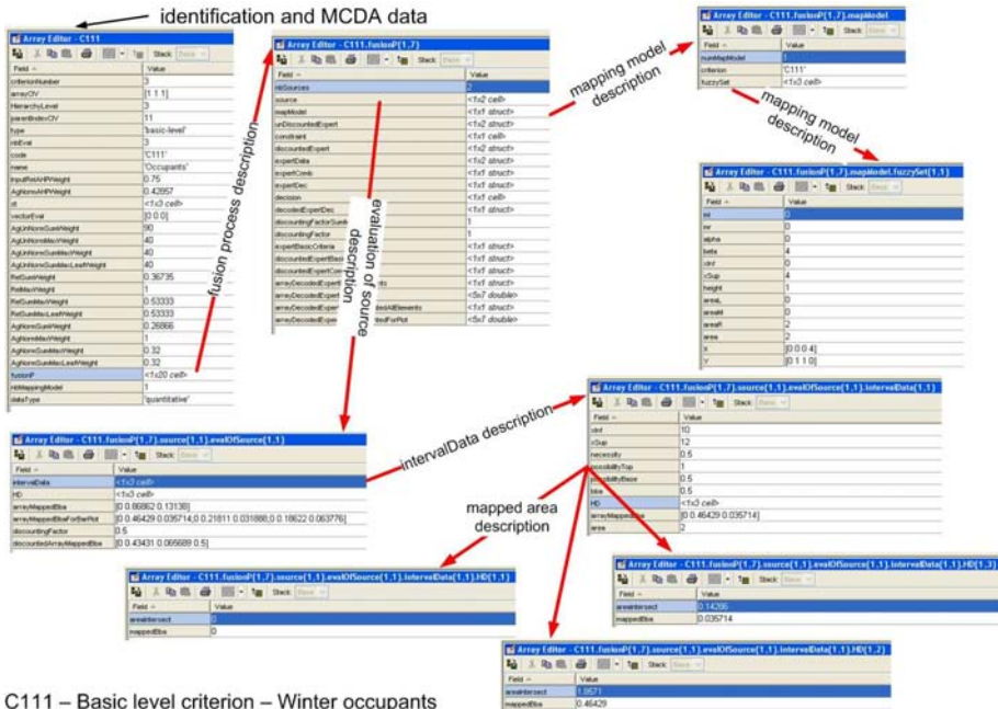
Figure 23.56: Quantitative criterion C_{[111]} - Fusion process no. 7 - Data structures from global identification to evaluation level.
