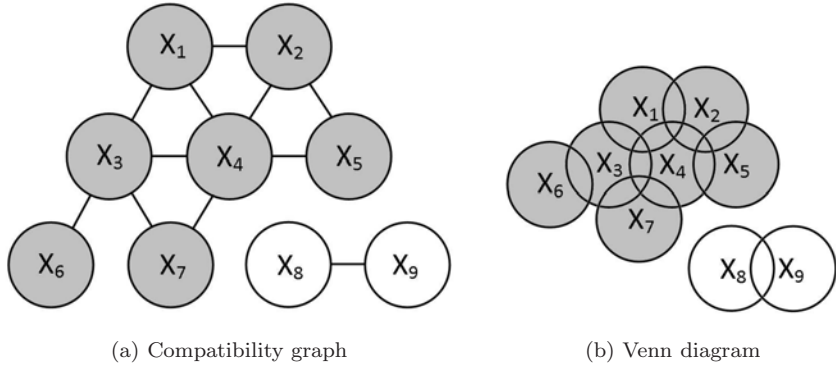
Figure 18.1: Building the frame of discernment from the compatibility graph. Hypotheses associated with cases in the same class are represented with the same color.
