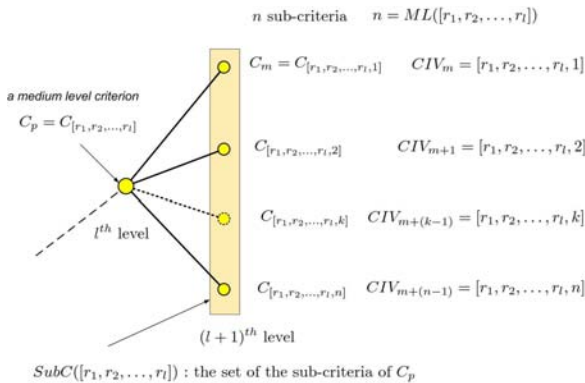
Figure 23.20: Criterion and sub-criteria codification in the hierarchical structure.
