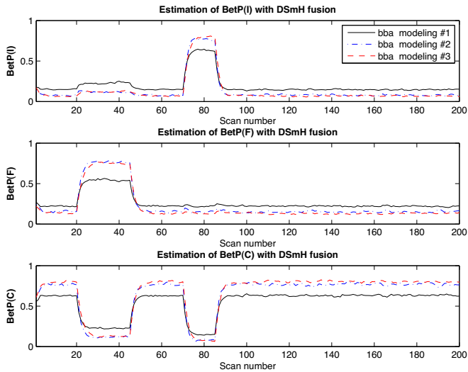
Figure 16.3: BetP(\cdot) results after using DS mH rule of combination.
