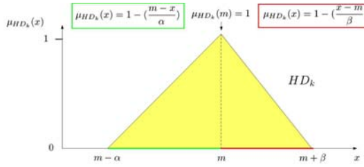
Figure 23.14: Fuzzy number L - R .
