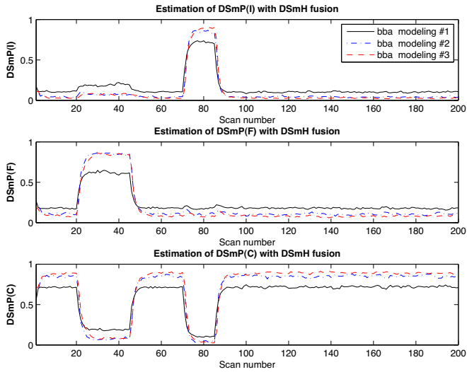
Figure 16.2: DSmP(\cdot) results after using DS mH rule of combination.
