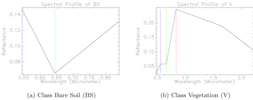
Figure 22.10: Spectral signatures of the classes Bare Soil (HRV 1997) and Vegetation (ETM+ 2001) in the variant site of the agricultural zone by the hybrid model.
