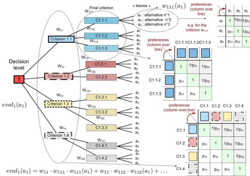
Figure 23.8: Principle of the Analytic Hierarchy Process (AHP).
