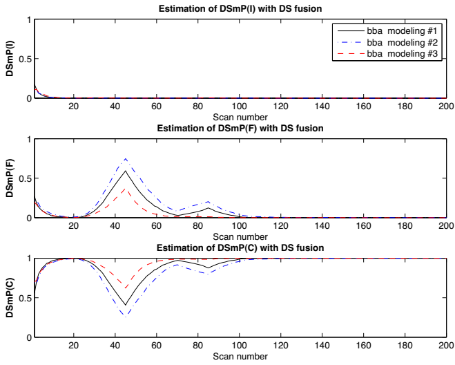
Figure 16.6: DSmP(.) results after using DS rule of combination.
