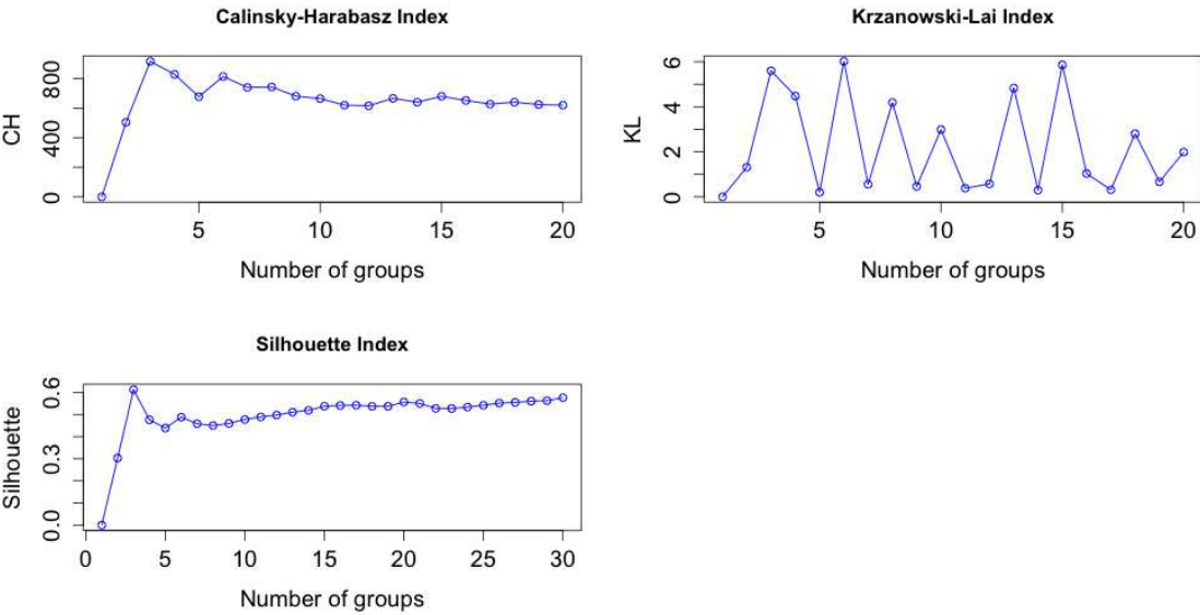
Figure 3: Partitioning quality indicators variations depending on the number of clusters
