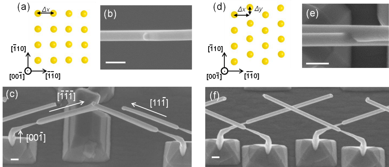
Figure 2. Position – and direction – controlled growth of InSb nanowire networks.
