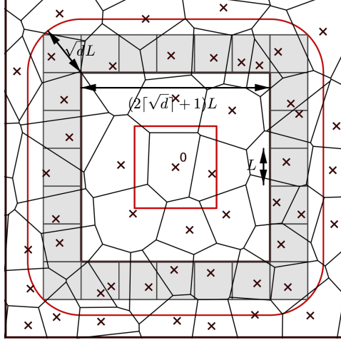
FIGURE 2. If each (grey) cube of side L that border [-(2\lceil\sqrt{d}\rceil + 1)L, (2\lceil\sqrt{d}\rceil + 1)L]^d contains at least a point of \xi^0 , then the nuclei of the Voronoi cells intersecting the boundary of [-(2\lceil\sqrt{d}\rceil + 1)L, (2\lceil\sqrt{d}\rceil + 1)L]^d lie in the region delimited by the red curves. In this case, the union of these cells surround 0 \in \xi^0 and the degree of 0 in \text{DT}(\xi^0) is bounded by \#([-4\lceil\sqrt{d}\rceil + 1)L, (4\lceil\sqrt{d}\rceil + 1)L]^d \cap \xi^0) .
