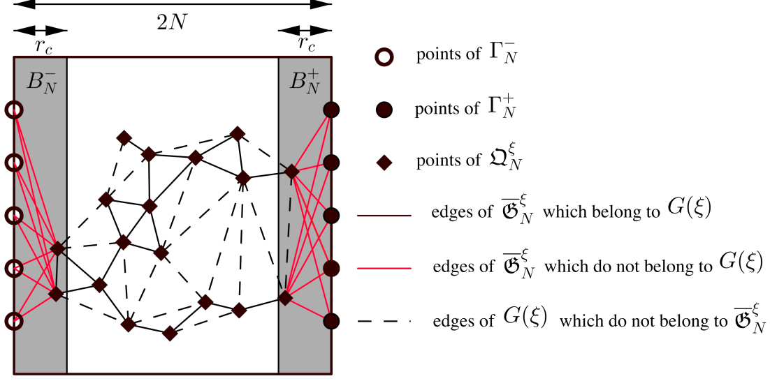
FIGURE 1. The vertex set of \overline{\mathfrak{G}}_N^\xi contains the points of \mathfrak{Q}_N^\xi = \xi \cap \mathring{C}_{2N} , \Gamma_N^- and \Gamma_N^+ . An edge of G(\xi) between points of \mathfrak{Q}_N^\xi is an edge of \overline{\mathfrak{G}}_N^\xi iff its Euclidean length is smaller than r_c . There is also an edge in \overline{\mathfrak{G}}_N^\xi between each point of \xi \cap B_N^- (resp. \xi \cap B_N^+ ) and each point of \Gamma_N^- (resp. \Gamma_N^+ ).
