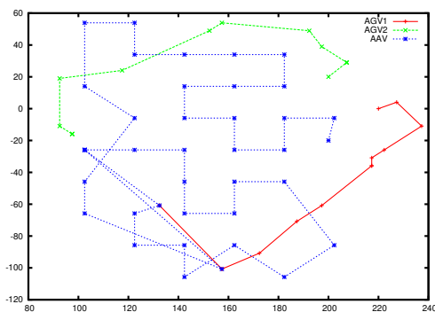
(b) Trajectories after greedy and local search
