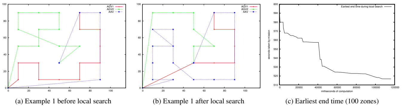
Figure 3: Plans produced on simple examples by the offline planning algorithm
