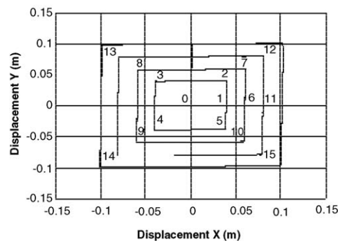
Fig. 6. R/C column: displacement load histories: (a) first test and (b) second test.
