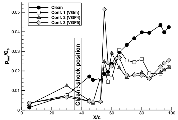
Fig. 9. Comparison of rms pressure distributions between the clean configuration and the controlled ones with mechanical and fluidic VGs ( \alpha = 3.5^\circ and M_0 = 0.82 )
