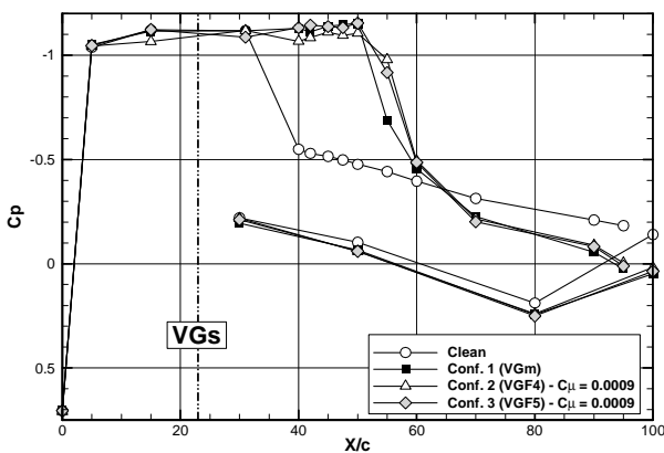
Fig. 8. Comparison of C_p distributions between the clean configuration and the controlled ones with mechanical and fluidic VGs ( \alpha = 3.5^\circ and M_0 = 0.82 )
