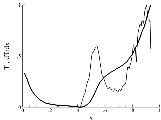
Fig. 16. Profile of temperature and its derivative as a function of chord-wise distance at M_0 = 0.73 and \alpha = 3.5^\circ
