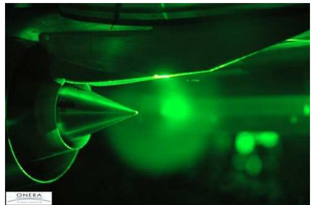
Fig. 4. Flow visualization by tomoscopy in the near wake of the nacelle
