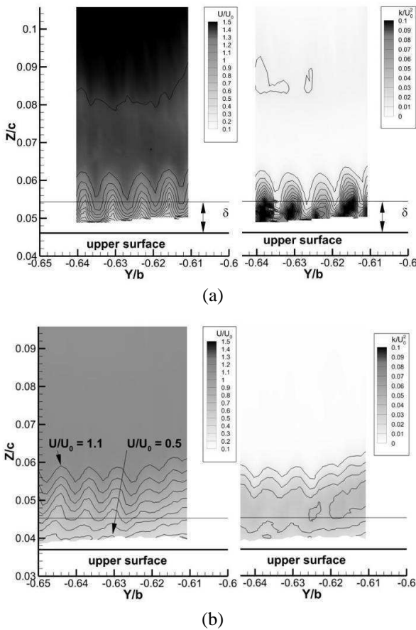
Fig. 10. Iso-values of the longitudinal velocity (left) and the turbulent kinetic energy (right) in the shock foot (a) and downstream of the shock (b), for the controlled configuration with fluidic VGs ( \alpha = 3.5^\circ and M_0 = 0.82 )
