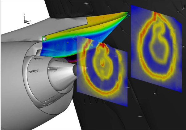
Fig. 5. TSP measurements on the pylon and LDV measurements in the near wake of the nacelle ( M_0 = 0.8 )
