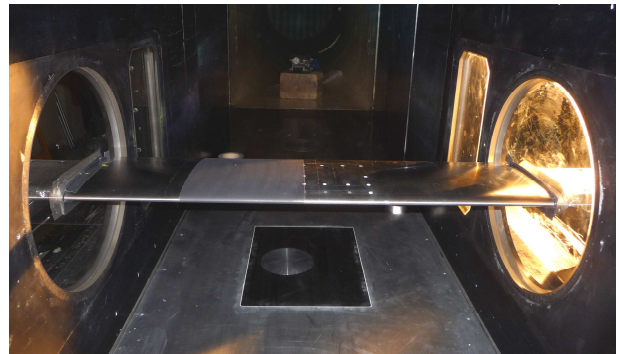
Fig. 12. View of the experimental set-up
