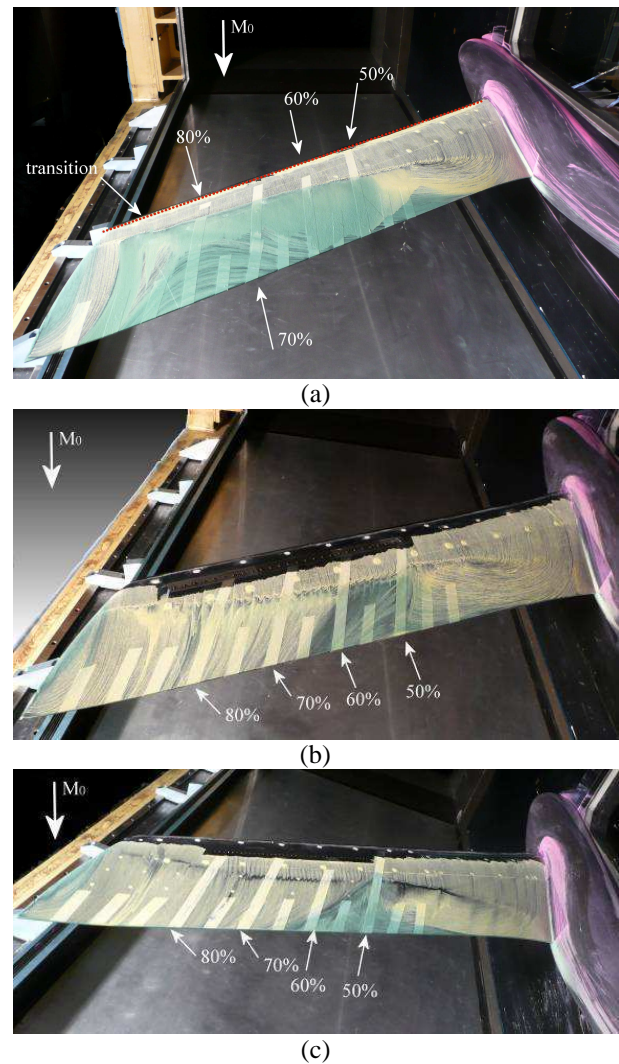
Fig. 7. Oil flow visualizations for the clean configuration (a) and the controlled ones with mechanical (b) and fluidic (c) VGs ( \alpha = 3.5^\circ and M_0 = 0.82 )
