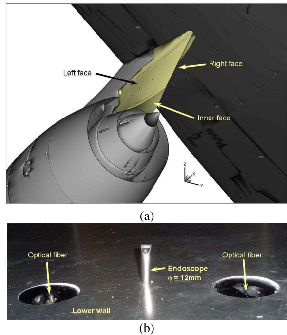
Fig. 3. Sketch of the pylon (a) and view of the endoscope mounted on the test section lower wall
