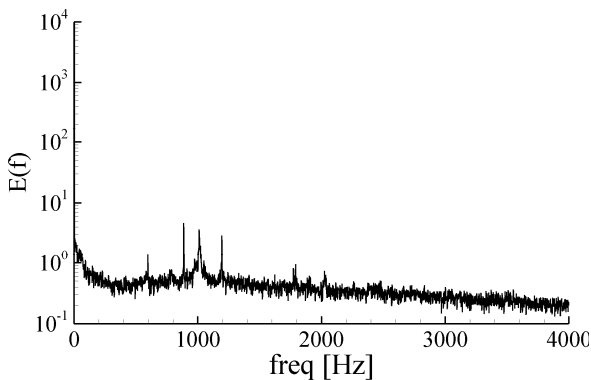
Fig. 14. Pressure spectrum obtained in the laminar condition at M_0 = 0.73 and \alpha = 3.5^\circ
