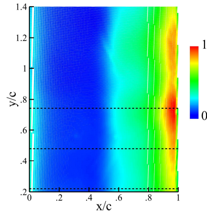
Fig. 15. Temperature distribution mapped to the range [0, 1] on the wing upper surface at M_0 = 0.73 and \alpha = 3.5^\circ
