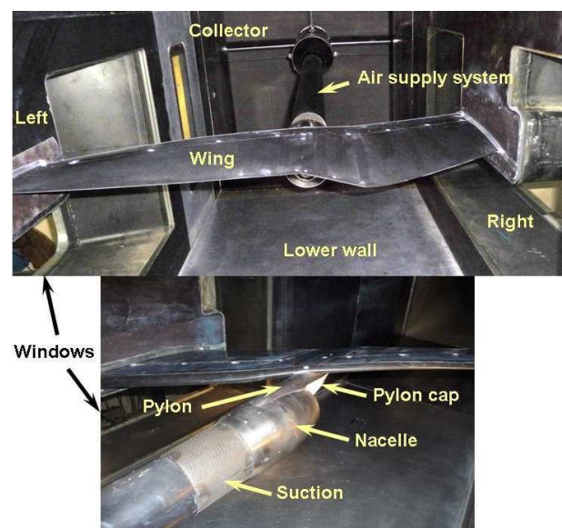
Fig. 2. View of the model and the air supply system upstream of the nacelle
