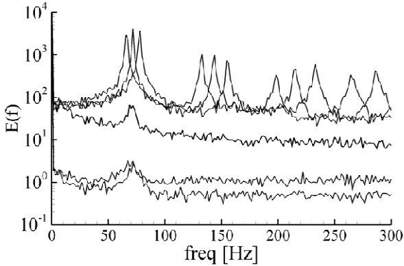
Fig. 13. Pressure spectra obtained in the turbulent condition at the shock foot at increasing Mach number 0.6, 0.68, 0.72, 0.73, 0.74 and 0.75 and \alpha = 3.5^\circ
