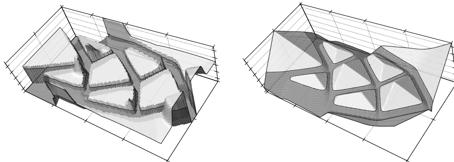
Figure 7: Level-set function for the 2-d cantilever without reinitialization (left) and with reinitialization (right)
