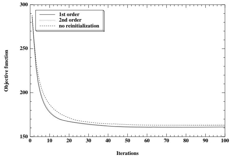
Figure 8: Convergence of the objective function for the two-dimensional cantilever of Figure 6 with various options
