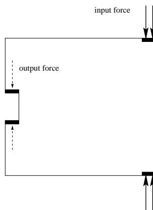
Figure 18: Boundary conditions for a plane gripping mechanism.
