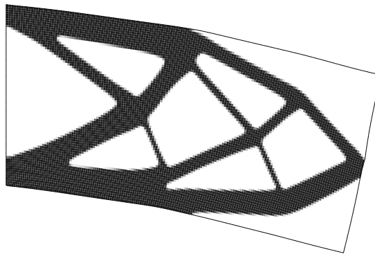
Figure 26: Optimal shape of a cantilever in nonlinear elasticity for different intensities of the force compared to the optimal shape in linear elasticity. Fine mesh ( 160 \times 80 ), initialized as in Figure 1 (middle)
