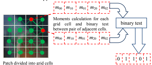
Figure 2: Illustration of MOBIL description algorithm.
