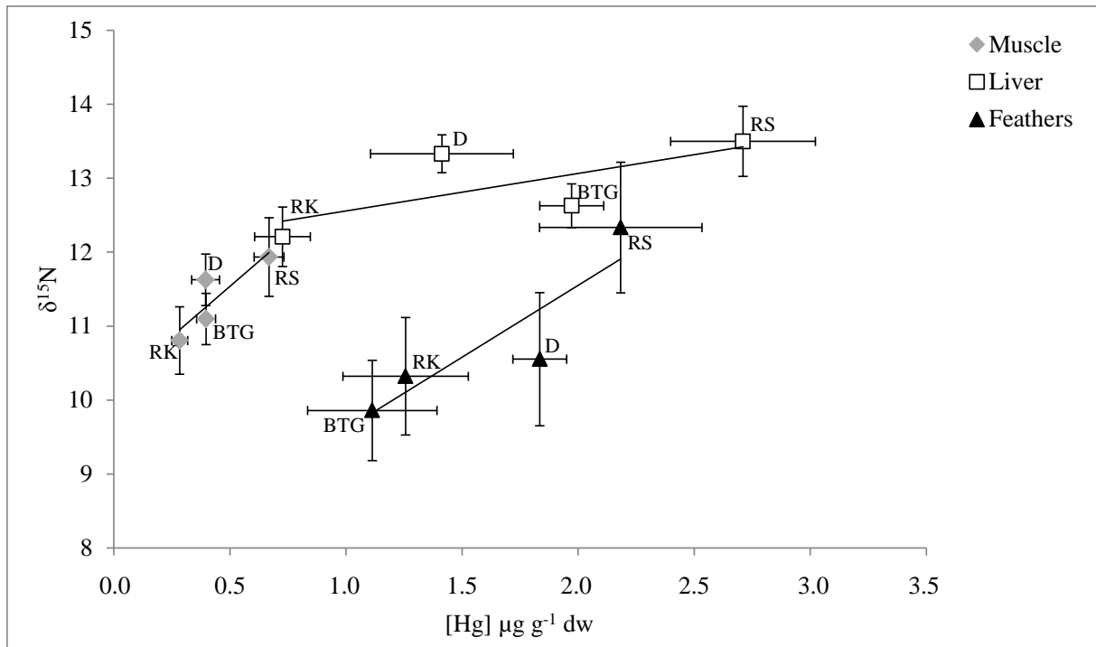
Fig. 4. Relationship between nitrogen ( \delta^{15}\text{N} ) isotopic signatures (mean ‰ \pm SE) and Hg concentrations ( \mu\text{g g}^{-1} \pm SE) in the liver, muscle and feathers of the Red Knot (RK), Black-tailed Godwit (BTG), Dunlin (D) and Redshank (RS) from the Pertuis Charentais.
