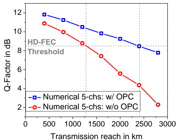
Fig. 6. Numerical simulations showing Q-factor versus reach of the link for the cases with and without OPC obtained at the optimum launch power levels.
